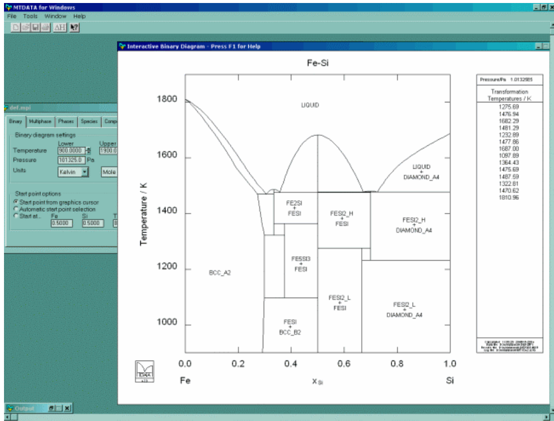
Figure 2: A binary diagram plotted using MTDATA for Windows
